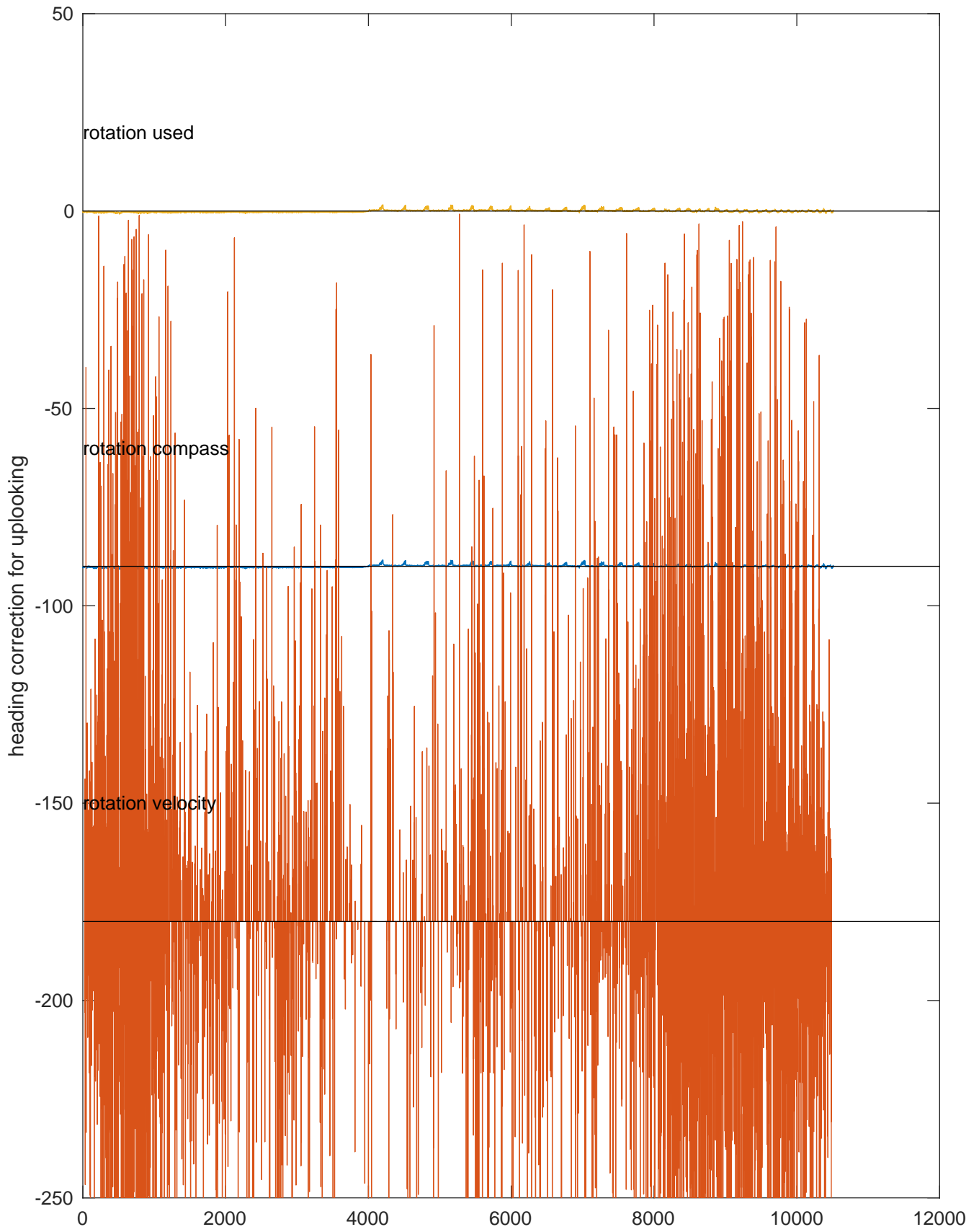
A22 station #45 (V3) Figure 5
