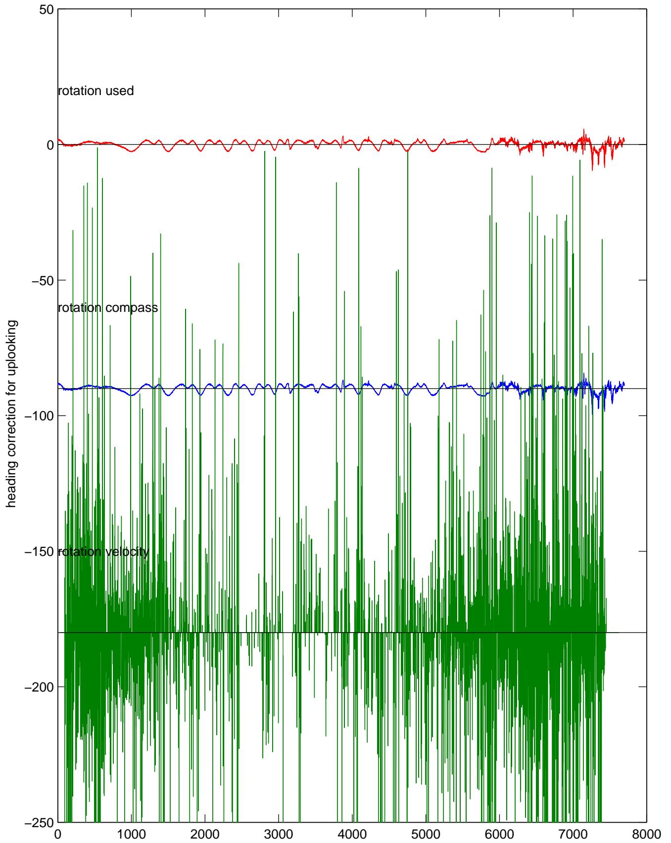
P16N station #16 (V7) Figure 5
