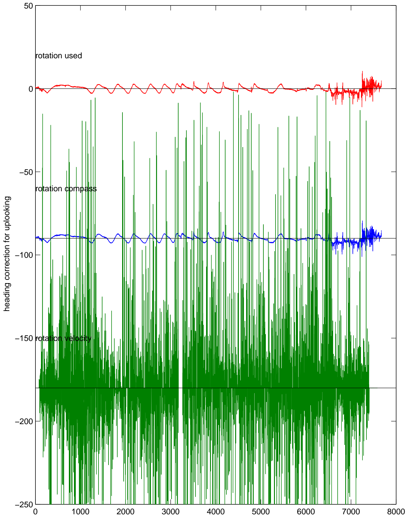
P16N station #46 (V7) Figure 5
