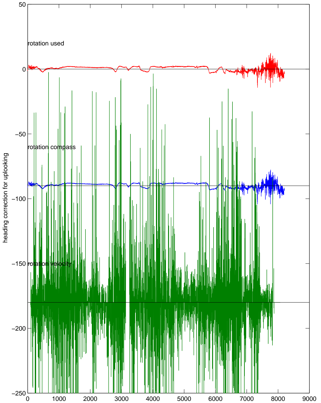
P16N station #53 (V7) Figure 5
