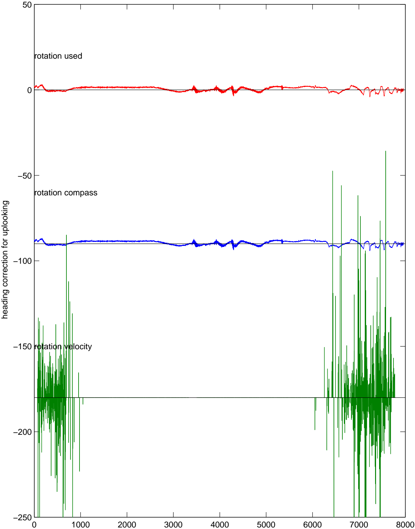
P16N station #130 (V7) Figure 5
