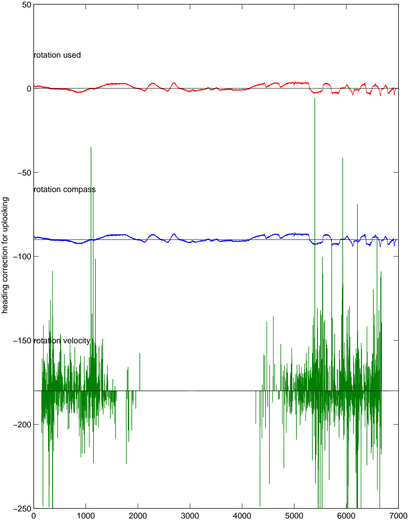
P16N station #171 (V7) Figure 5
