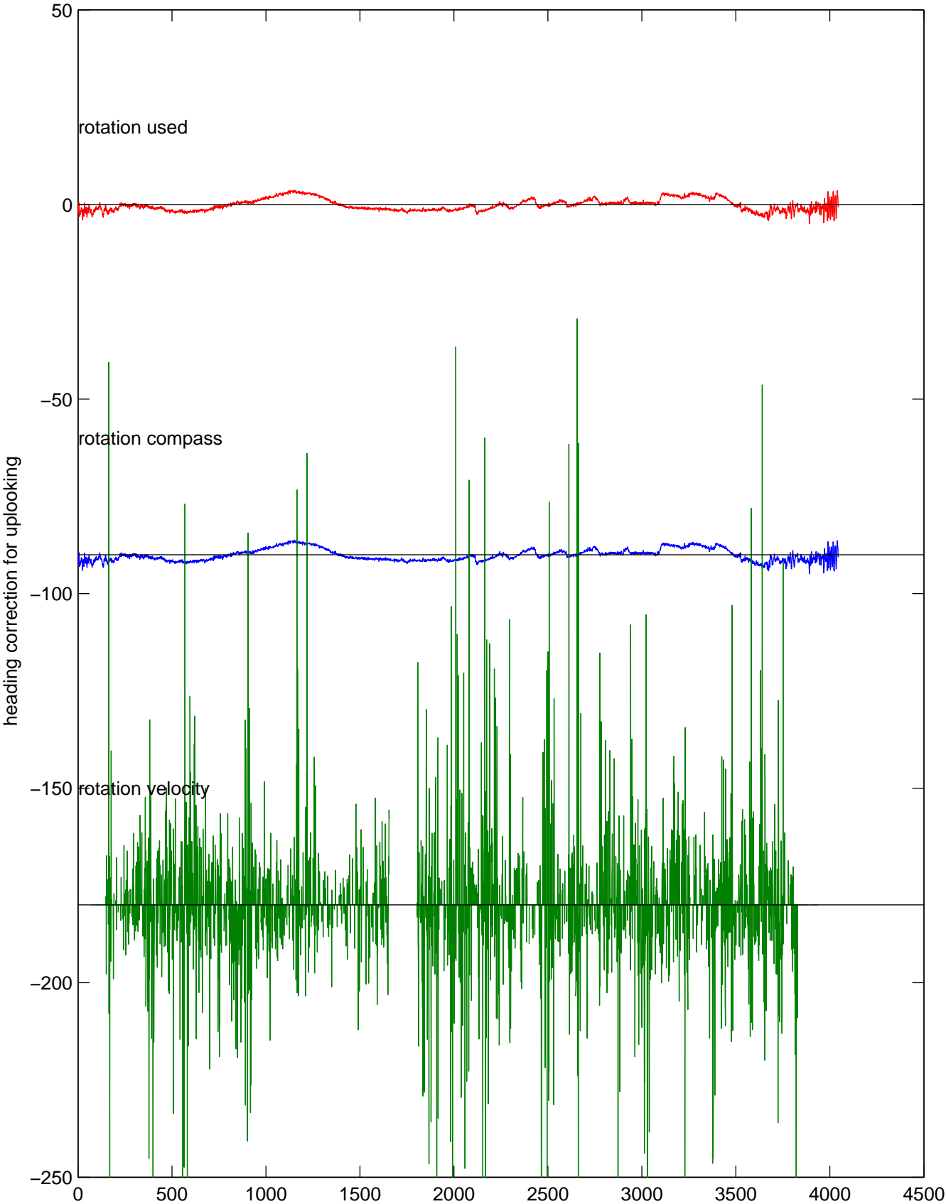
P16N station #190 (V7) Figure 5
