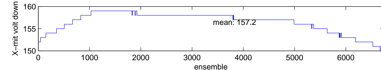
Beam Performance
