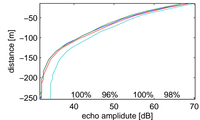
Beam Performance
