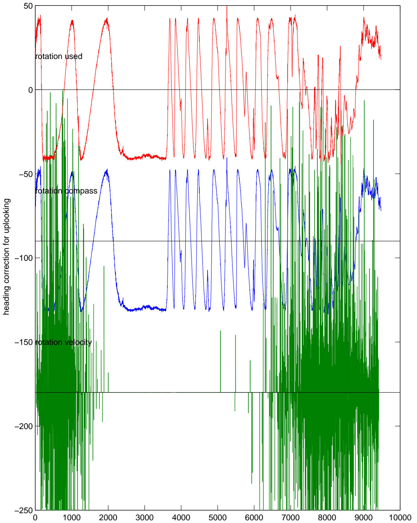
I08S station #95 (V2) Figure 5
