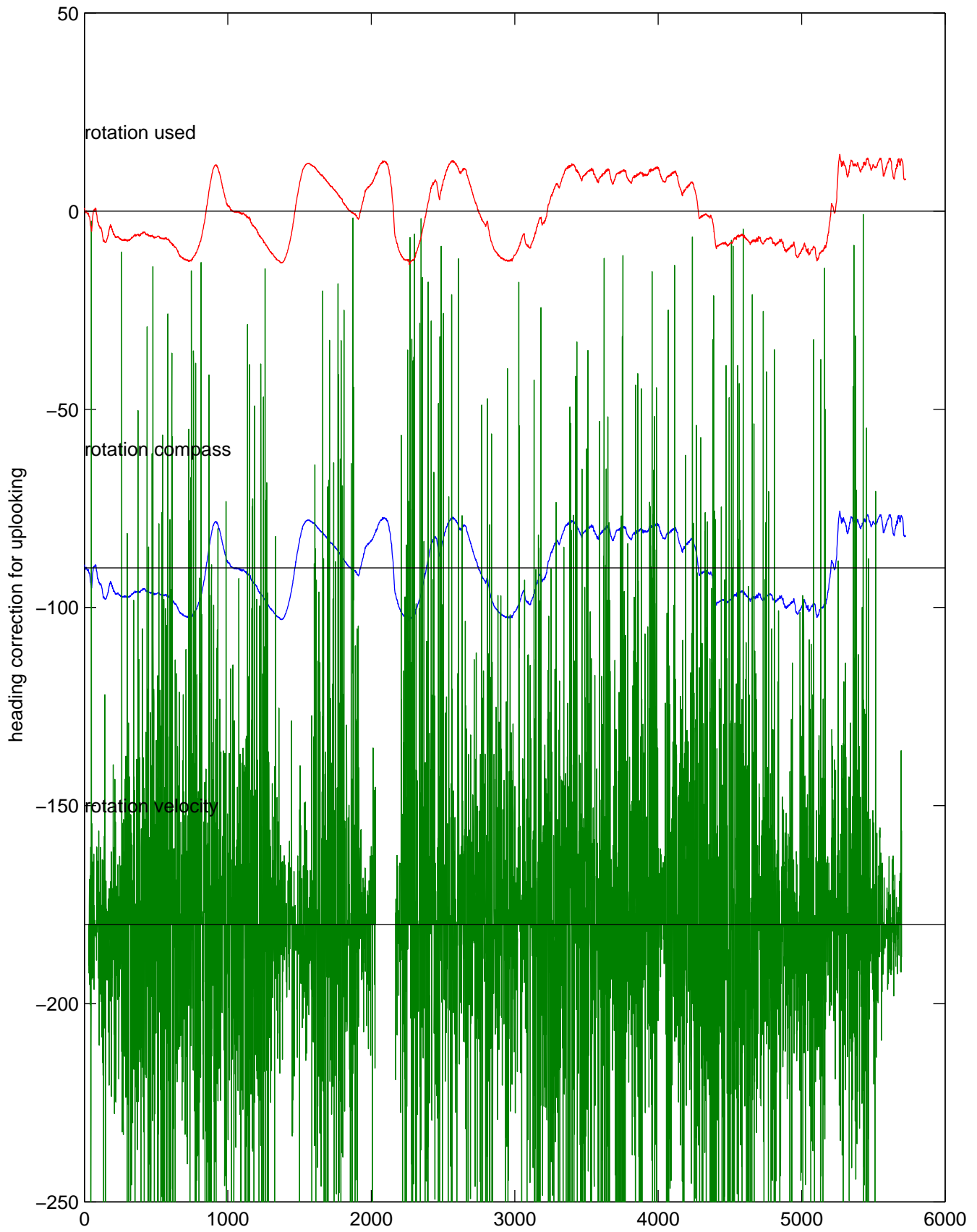
I08S station #156 (V2) Figure 5
