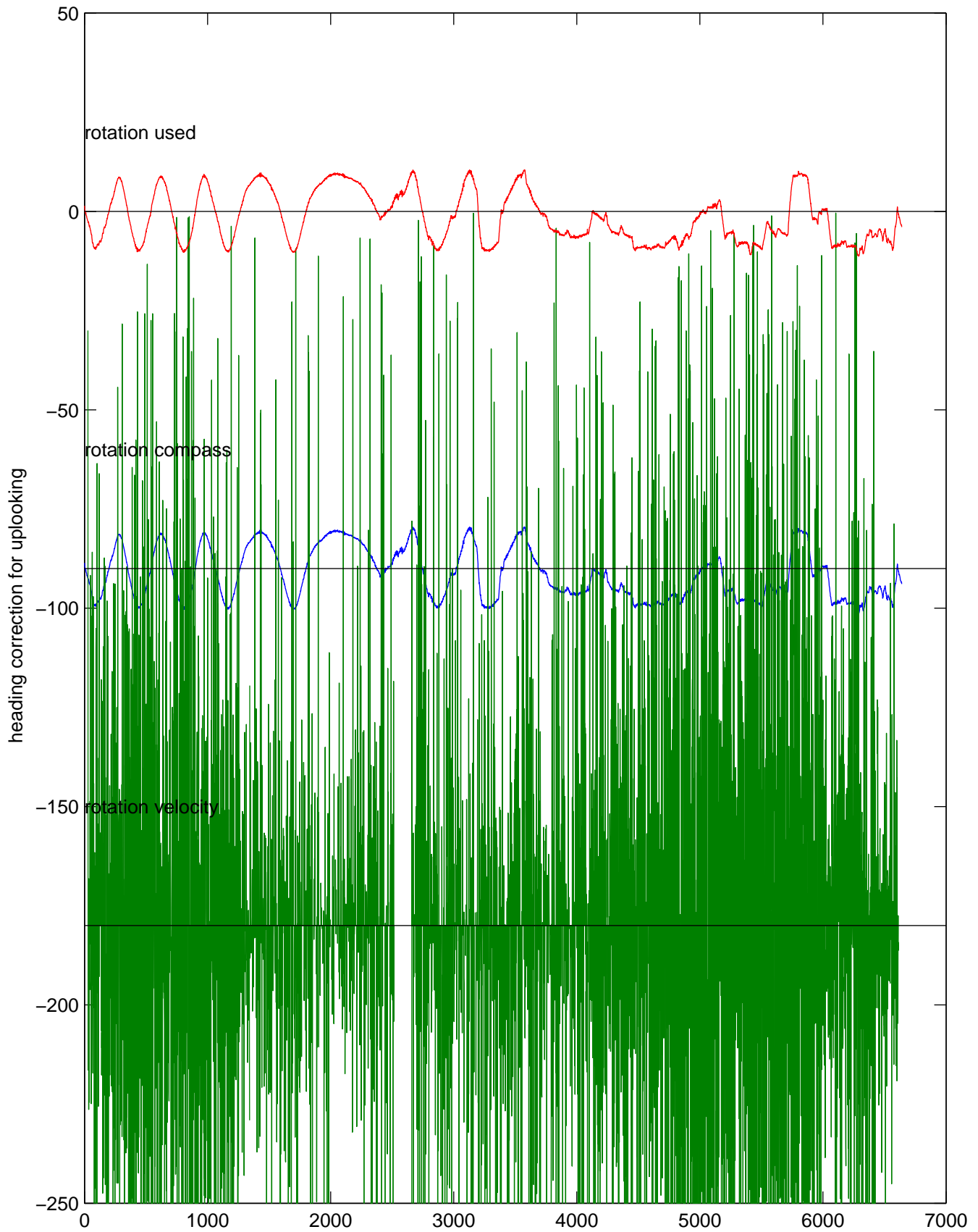
I08S station #168 (V2) Figure 5
