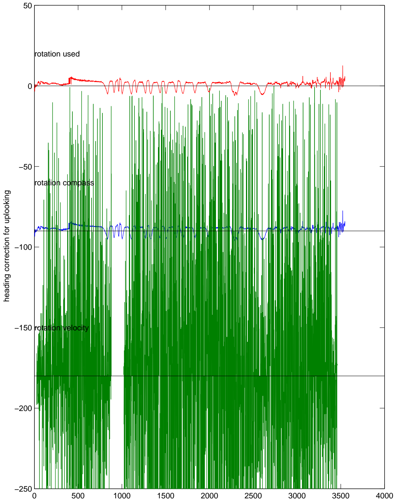
rh10031 (LADCP #010; V5) Figure 5
