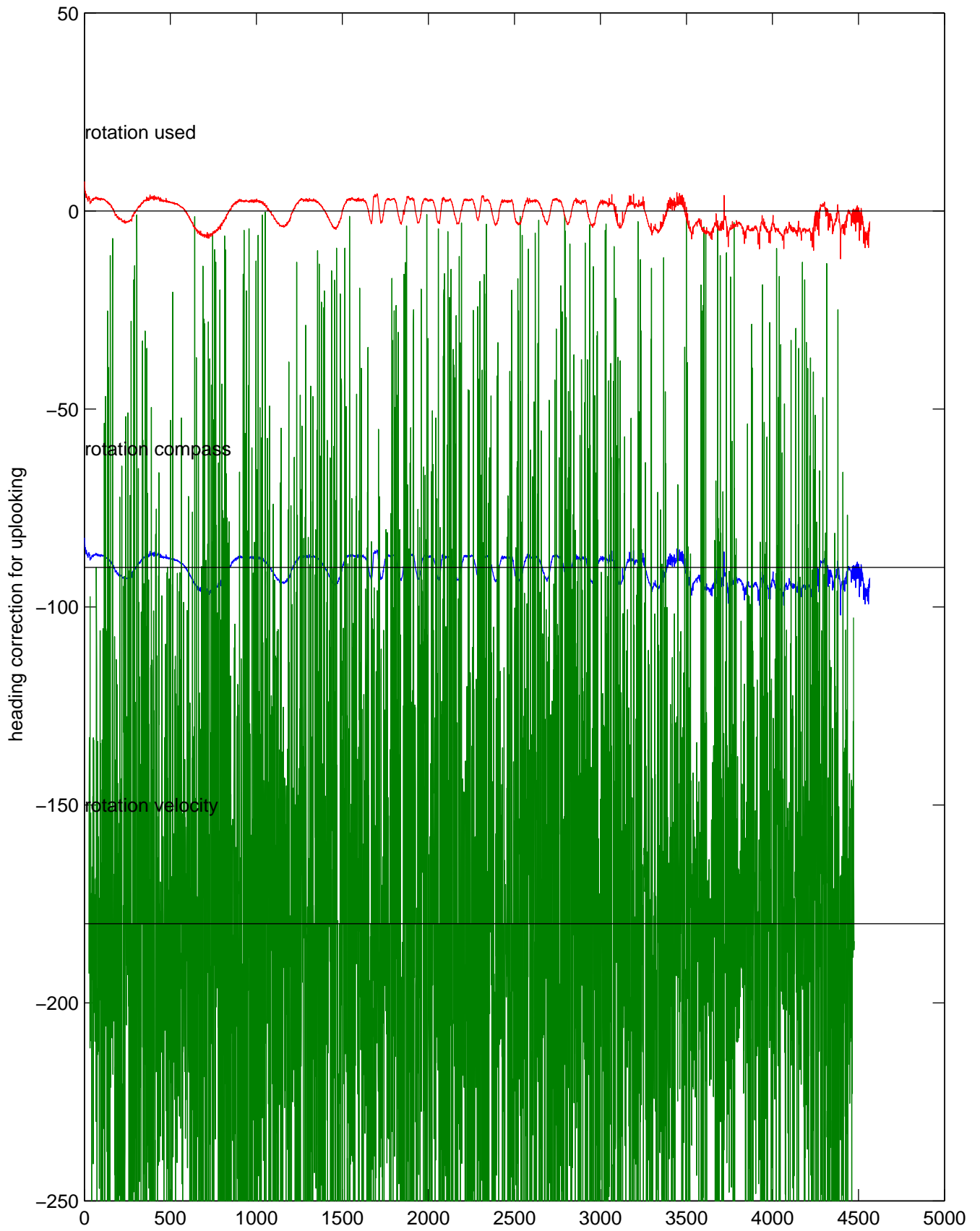
rh10091 (LADCP #016; V5) Figure 5
