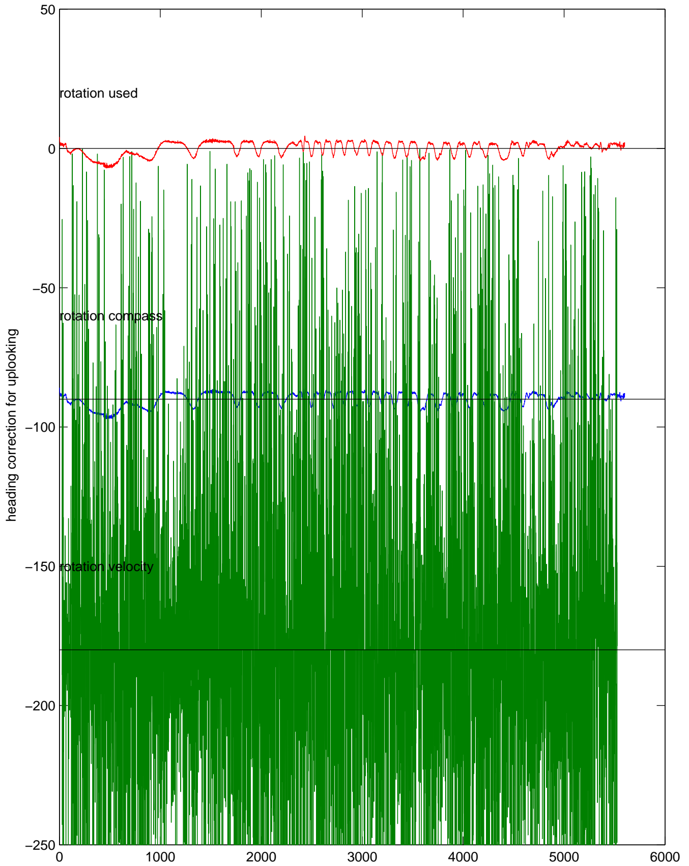
rh10211 (LADCP #029; V5) Figure 5
