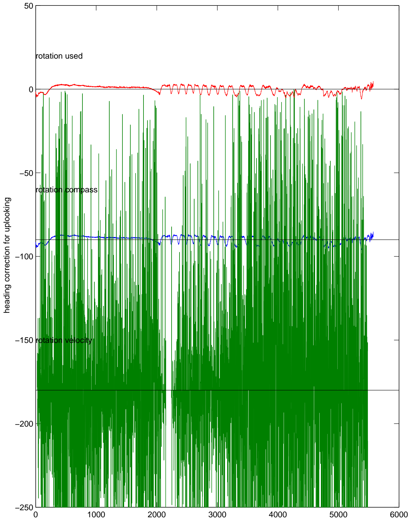
rh10231 (LADCP #031; V5) Figure 5
