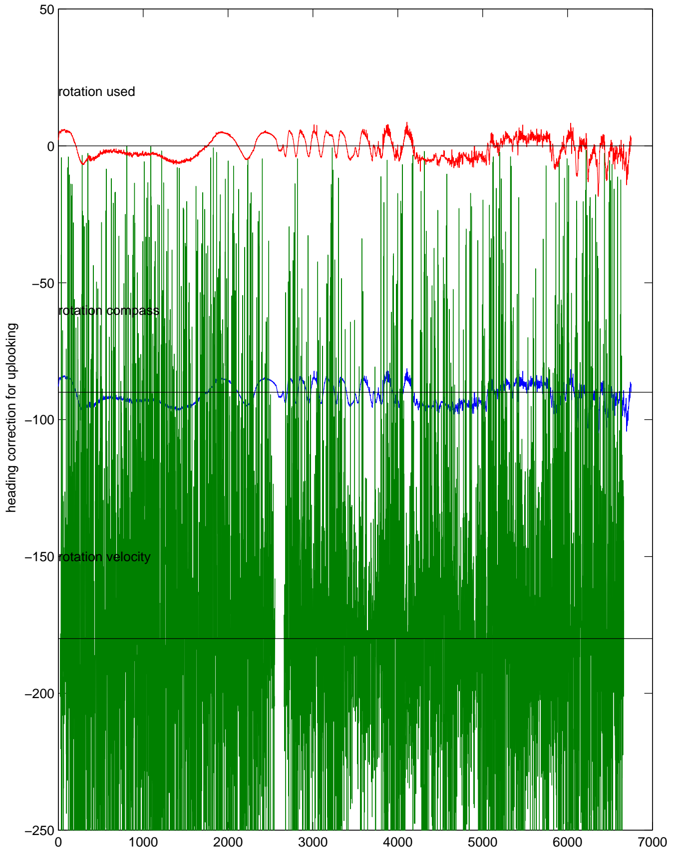
rh10381 (LADCP #046; V5) Figure 5
