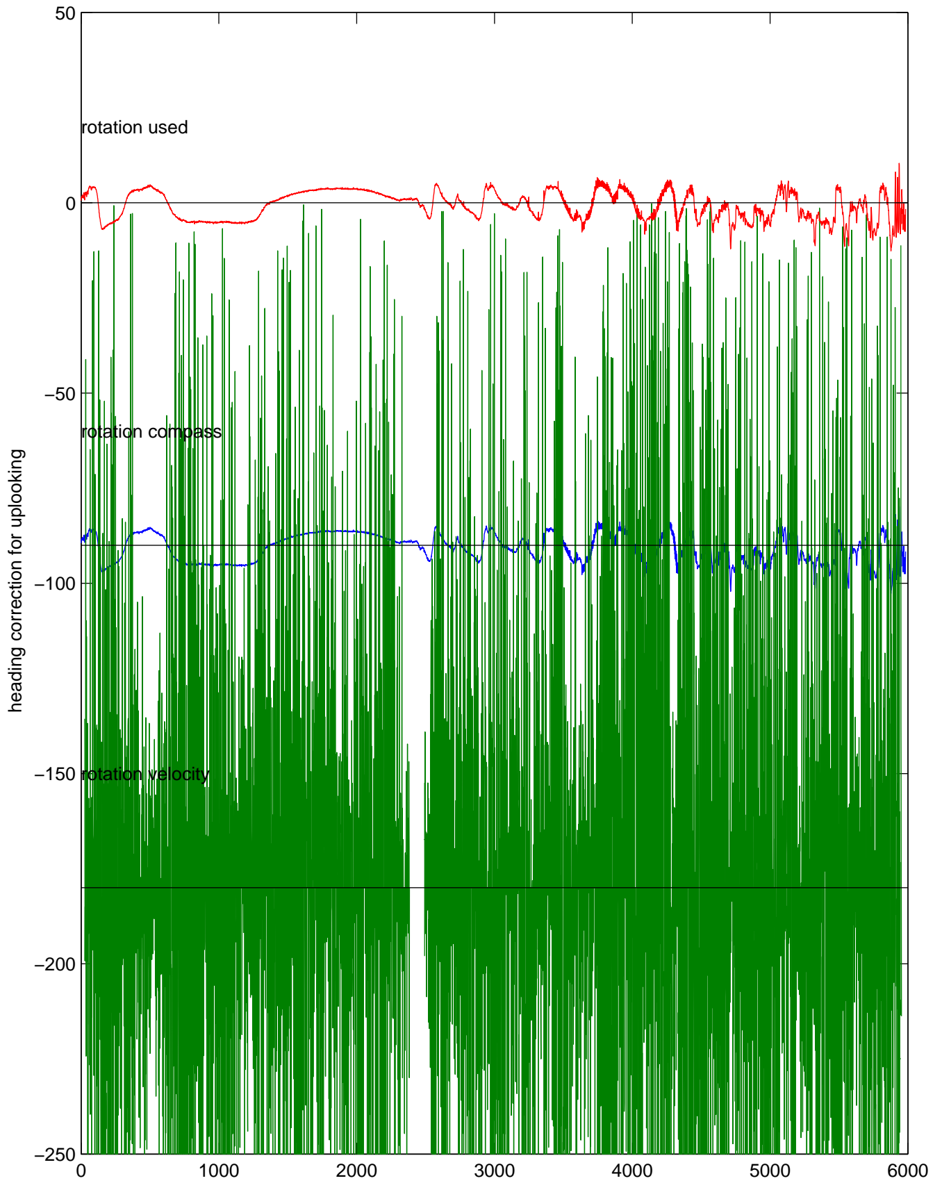
rh10501 (LADCP #058; V5) Figure 5
