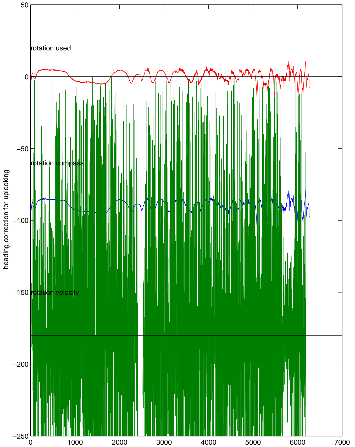
rh10661 (LADCP #074; V5) Figure 5
