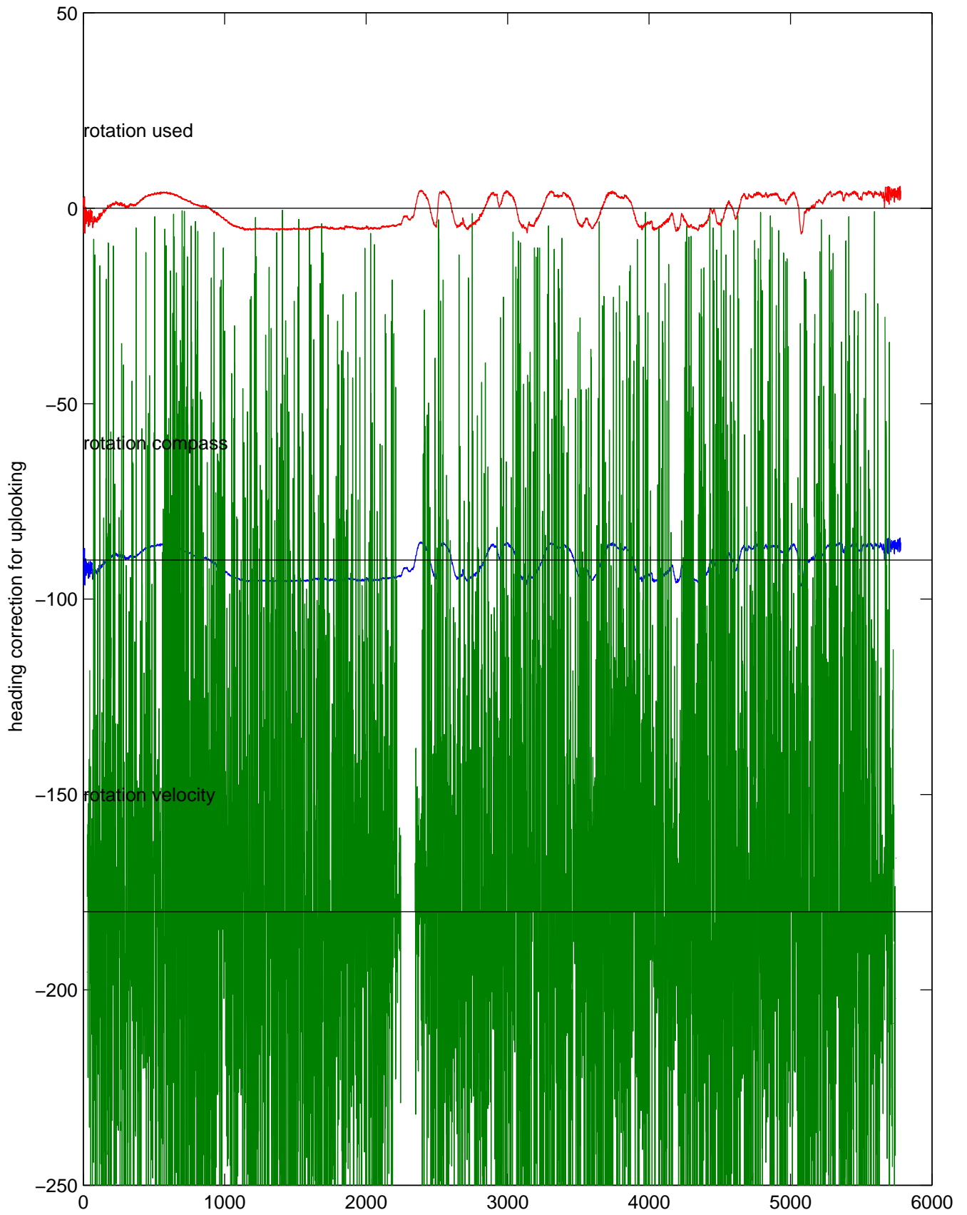
rh10701 (LADCP #078; V5) Figure 5
