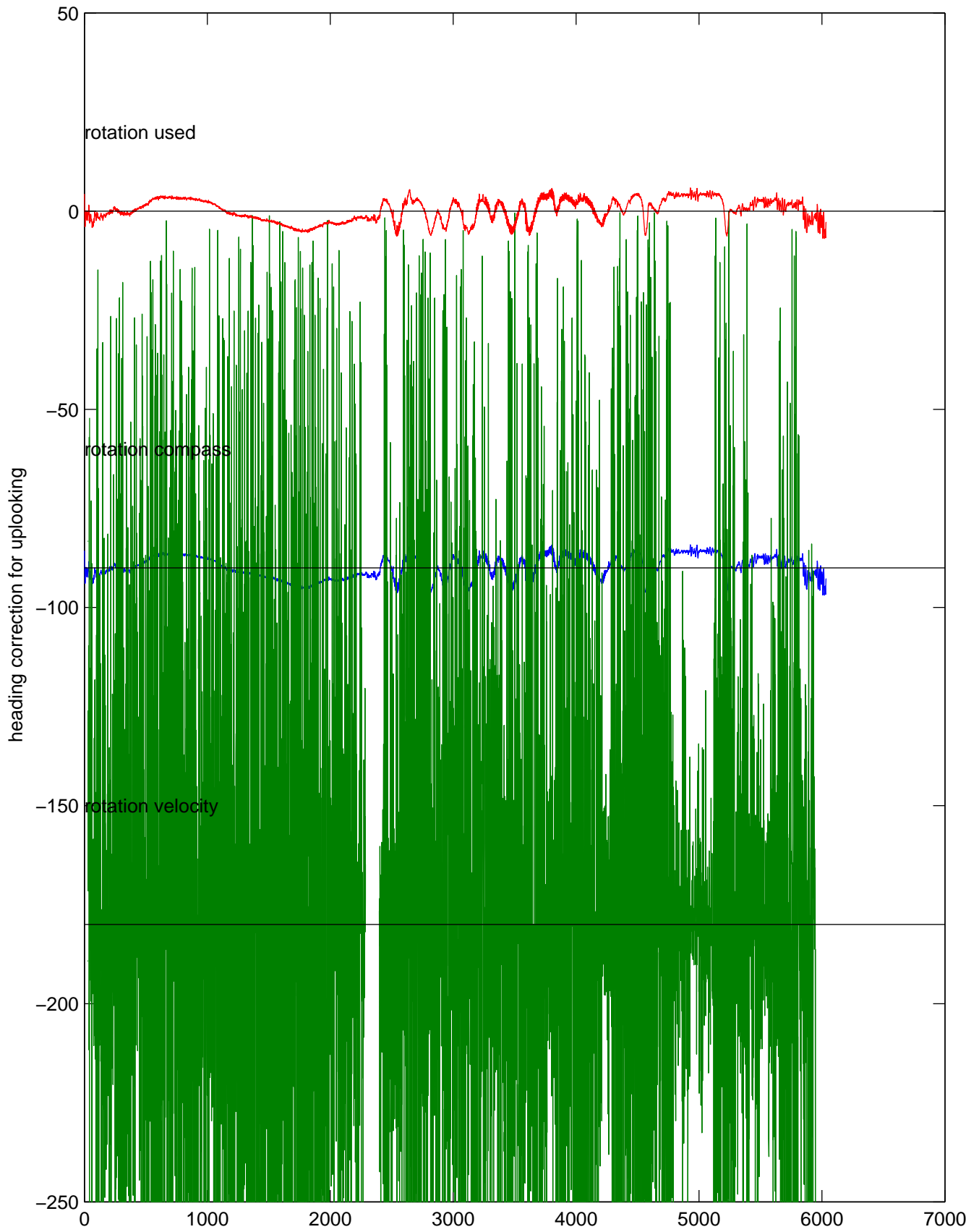
rh10711 (LADCP #079; V5) Figure 5
