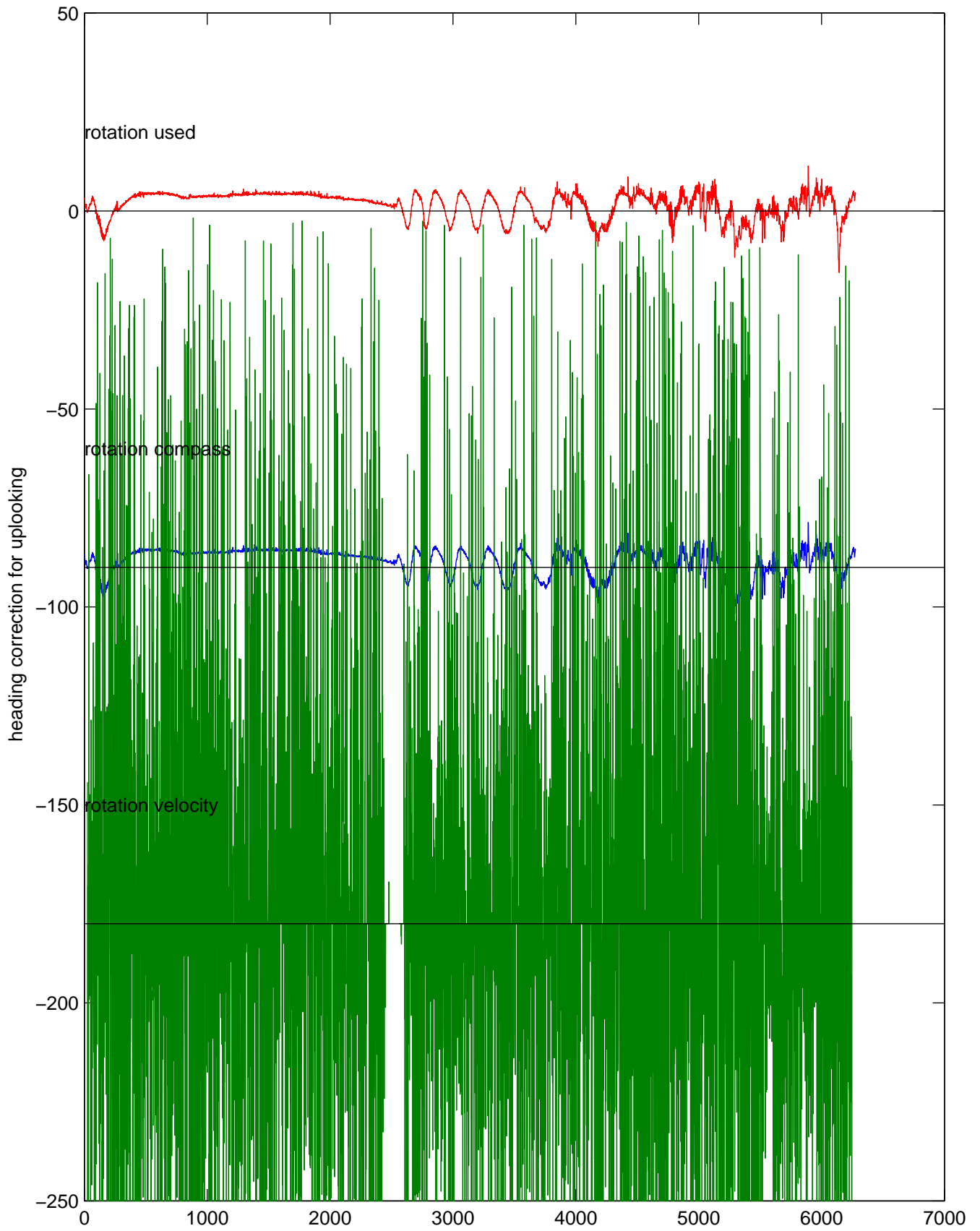
rh11031 (LADCP #111; V5) Figure 5
