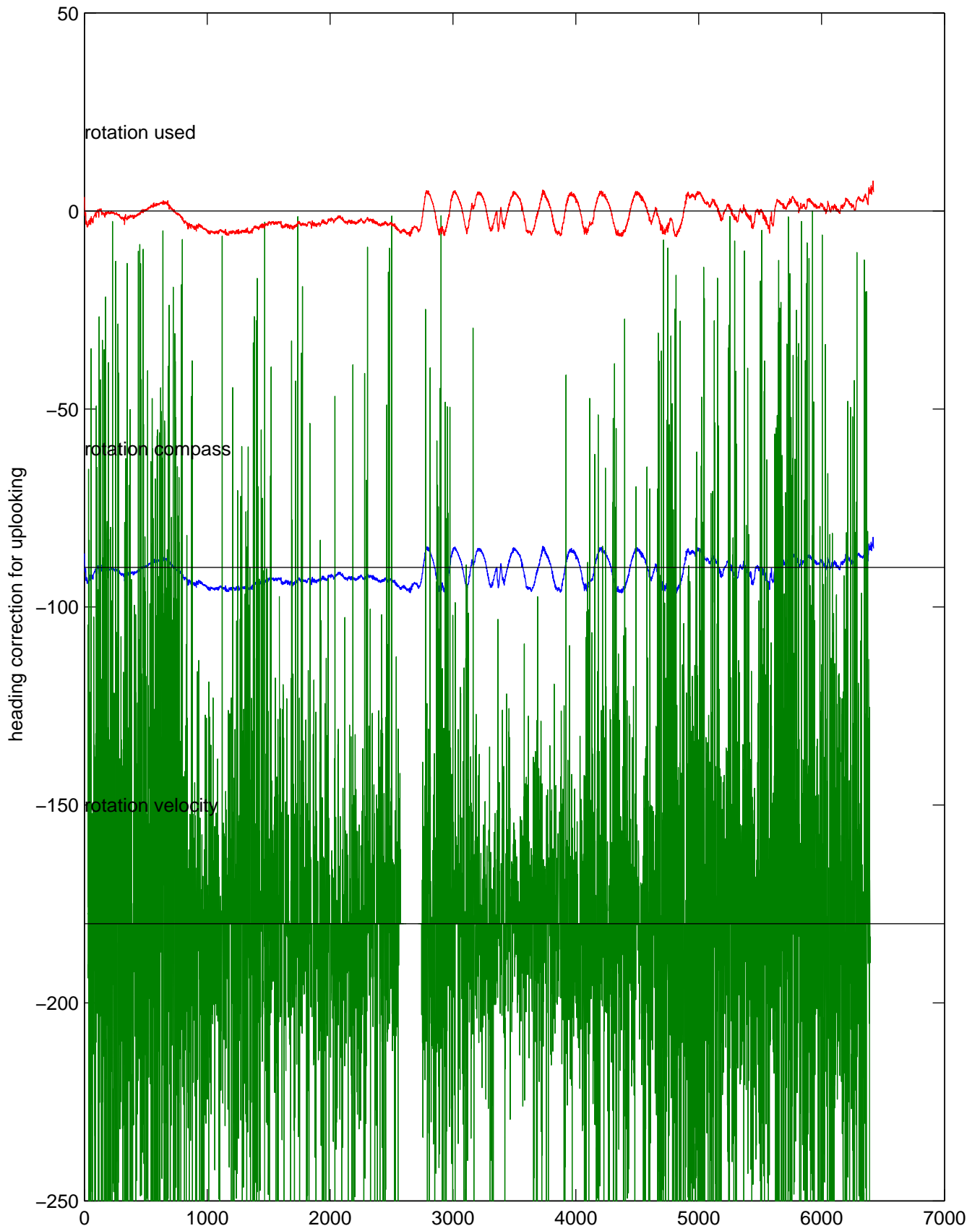
rh11061 (LADCP #114; V5) Figure 5
