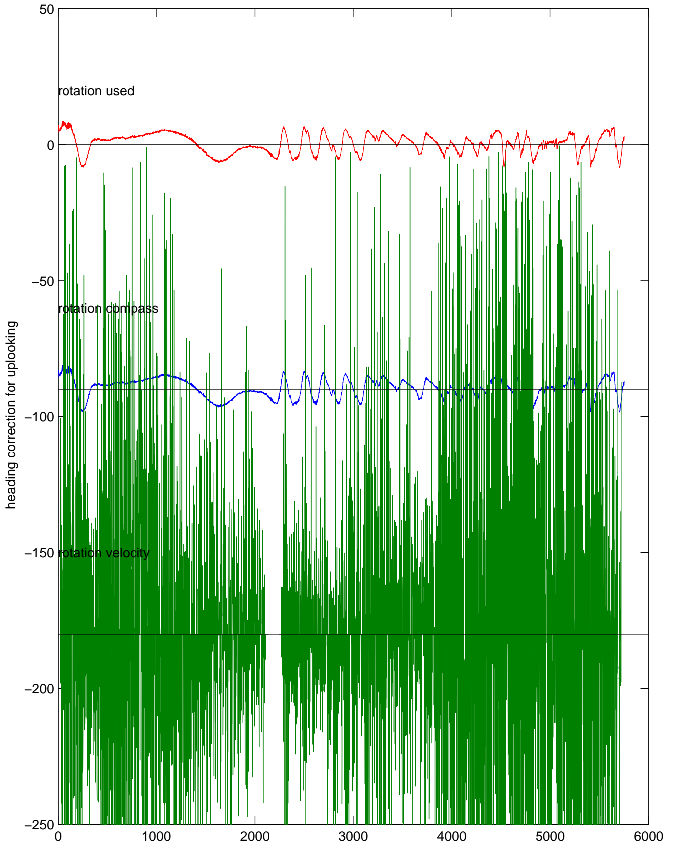
rh11271 (LADCP #137; V5) Figure 5
