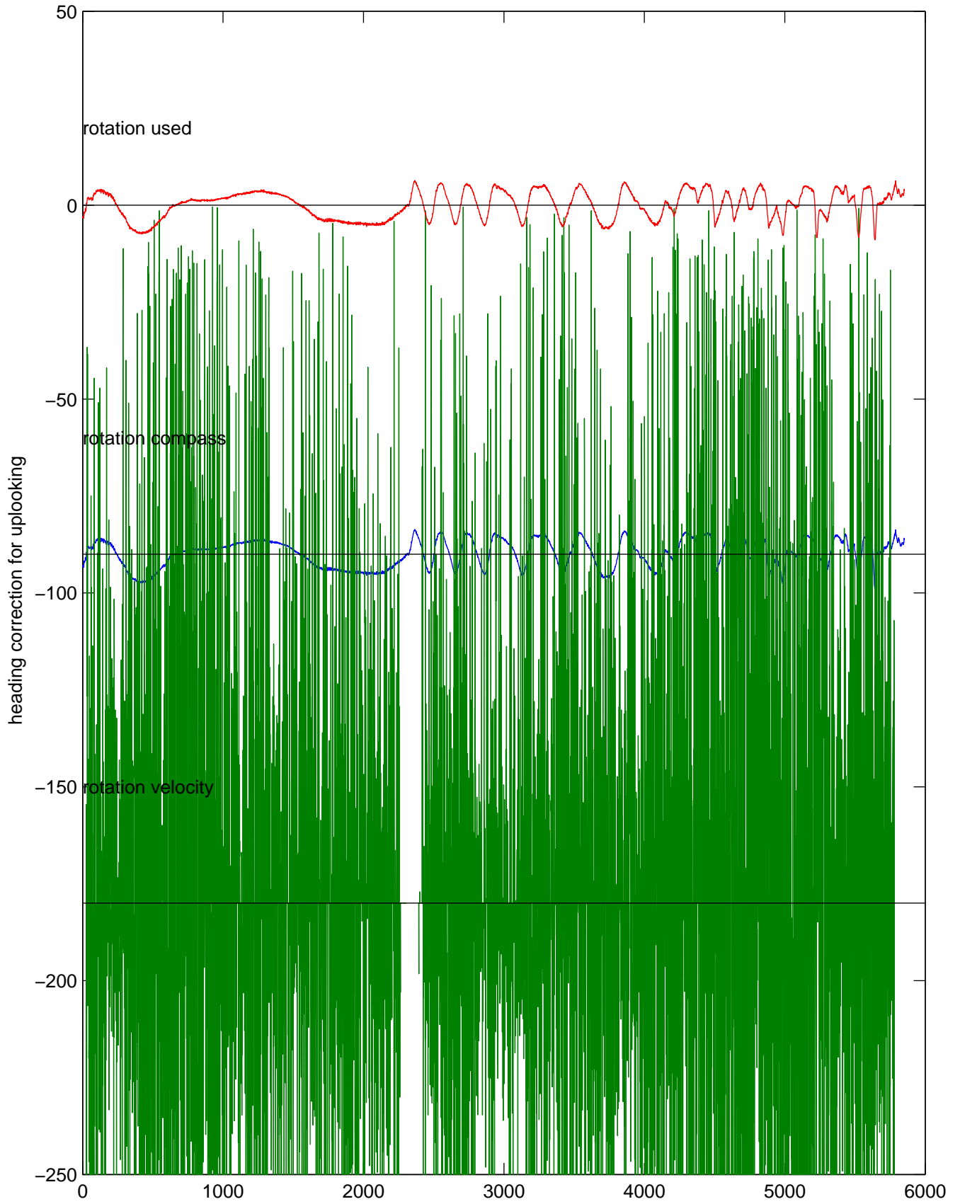
rh11321 (LADCP #144; V5) Figure 5
