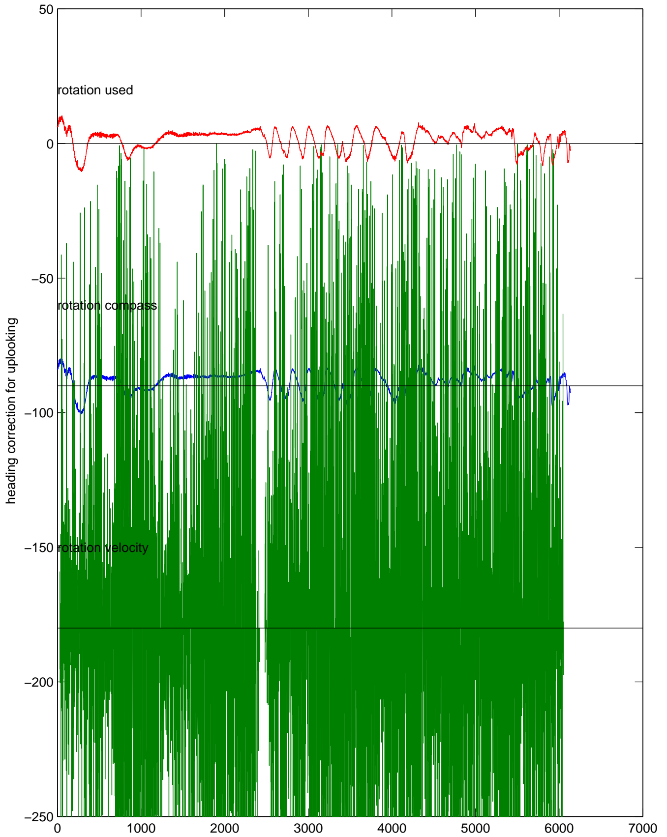
rh11401 (LADCP #152; V5) Figure 5
