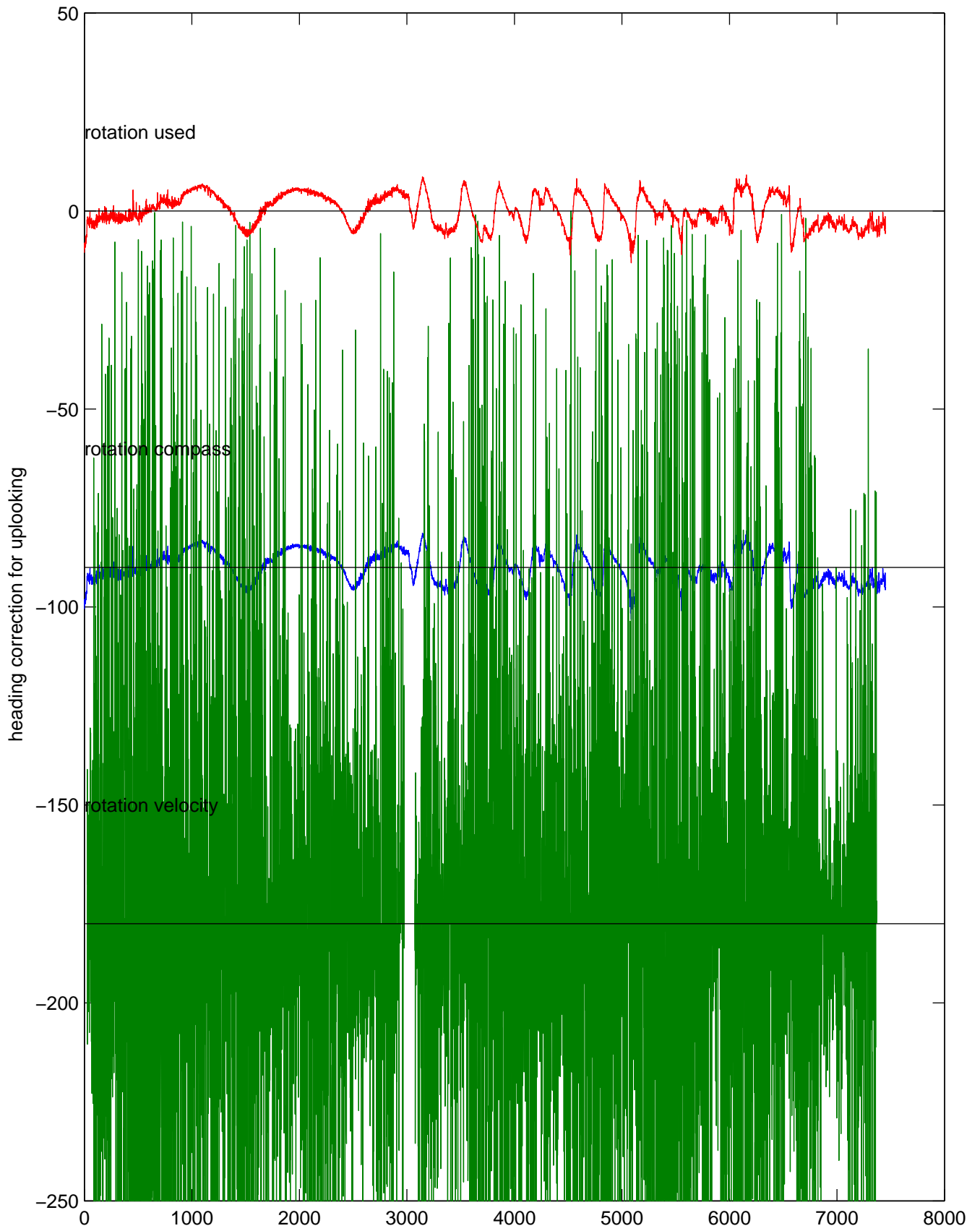
rh11851 (LADCP #198; V5) Figure 5
