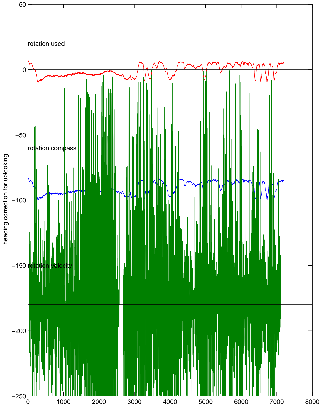
rh12061 (LADCP #221; V5) Figure 5
