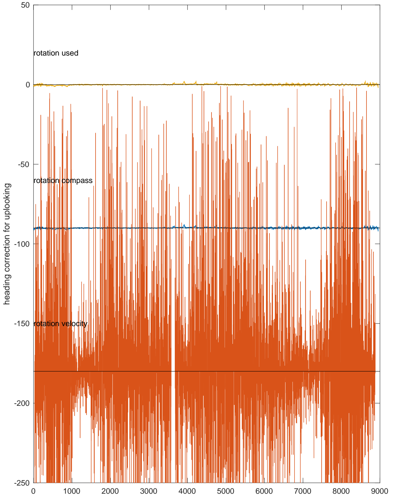
A20 station #73 (V7) Figure 5
