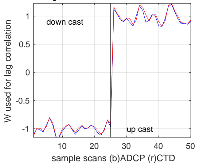
best lag W: 31 scans ~ -31 sec. c:0.99698
