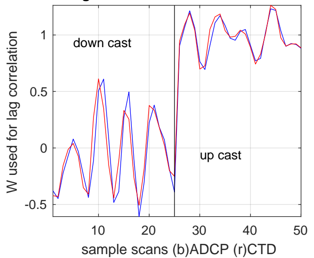
best lag W: 31 scans ~ -31 sec. c:0.99452
