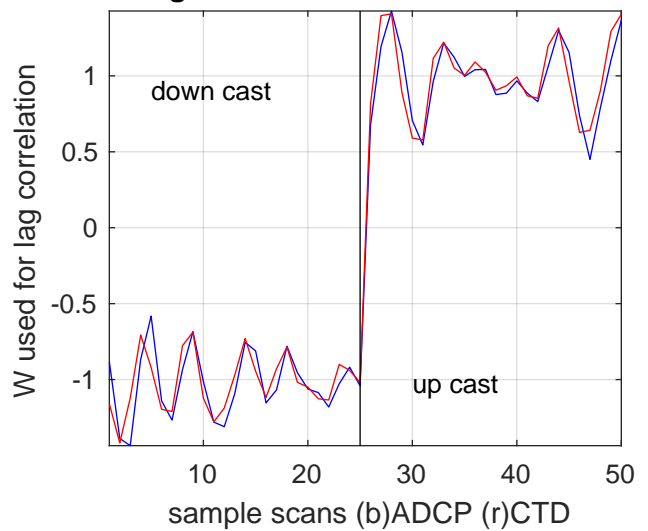
best lag W: 19 scans ~ -19 sec. c:0.99257
