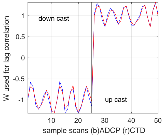
best lag W: 25 scans ~ -25 sec. c:0.99338
