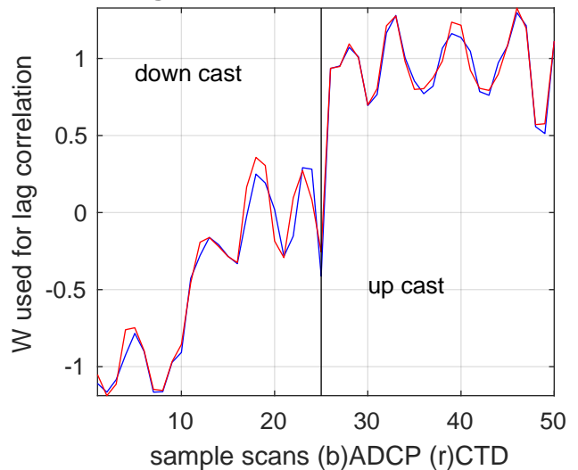
best lag W: 28 scans ~ -28 sec. c:0.99491
