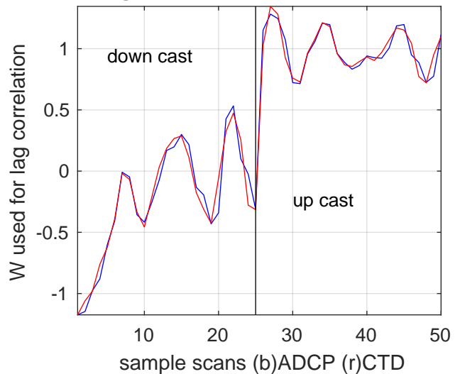
best lag W: 29 scans ~ -29 sec. c:0.99446
