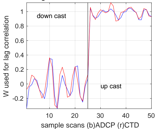
best lag W: 26 scans ~ -26 sec. c:0.99409
