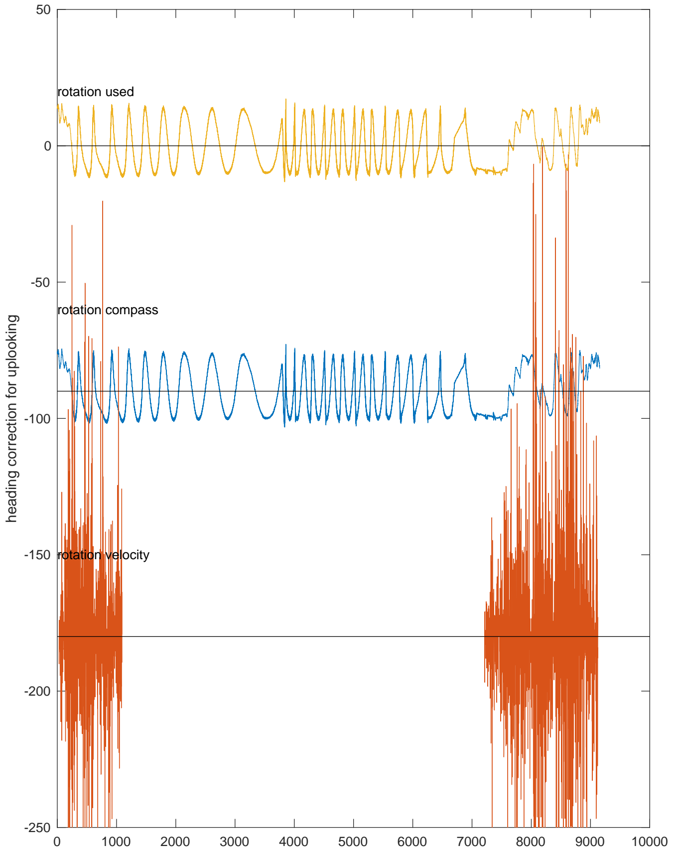
P2E station #9401 (V7) Figure 5
