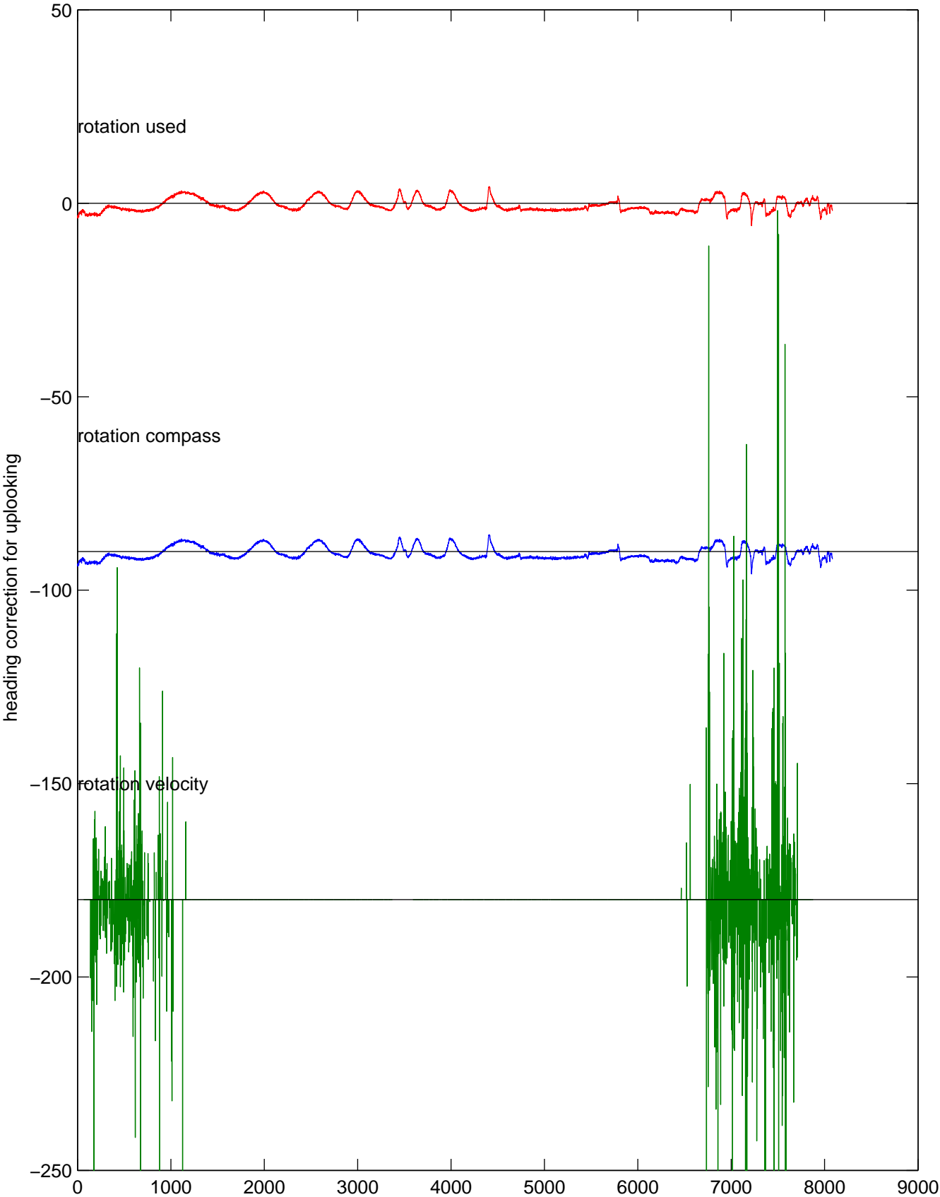
P16N station #136 (V7) Figure 5
