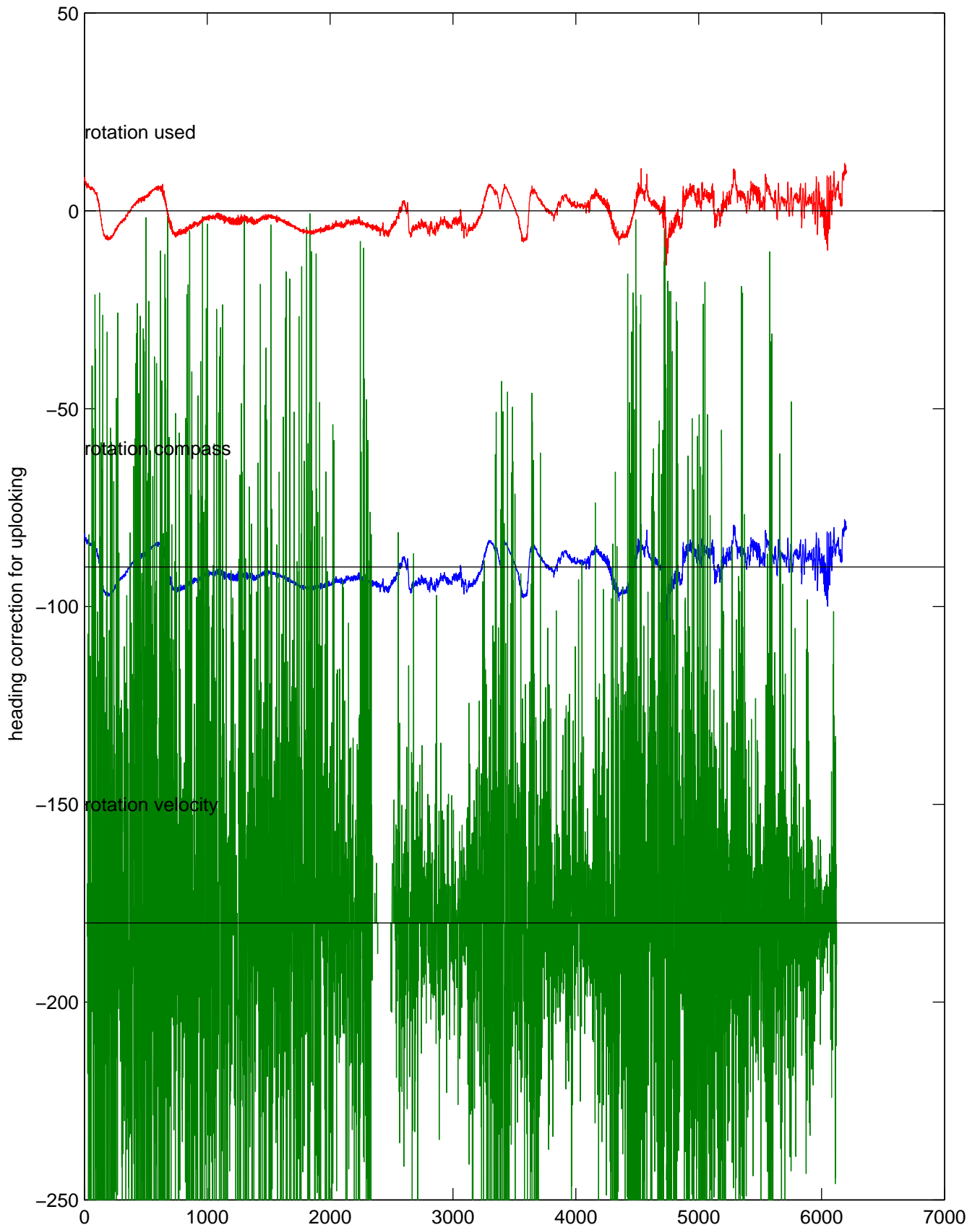
rh11531 (LADCP #165; V5) Figure 5
