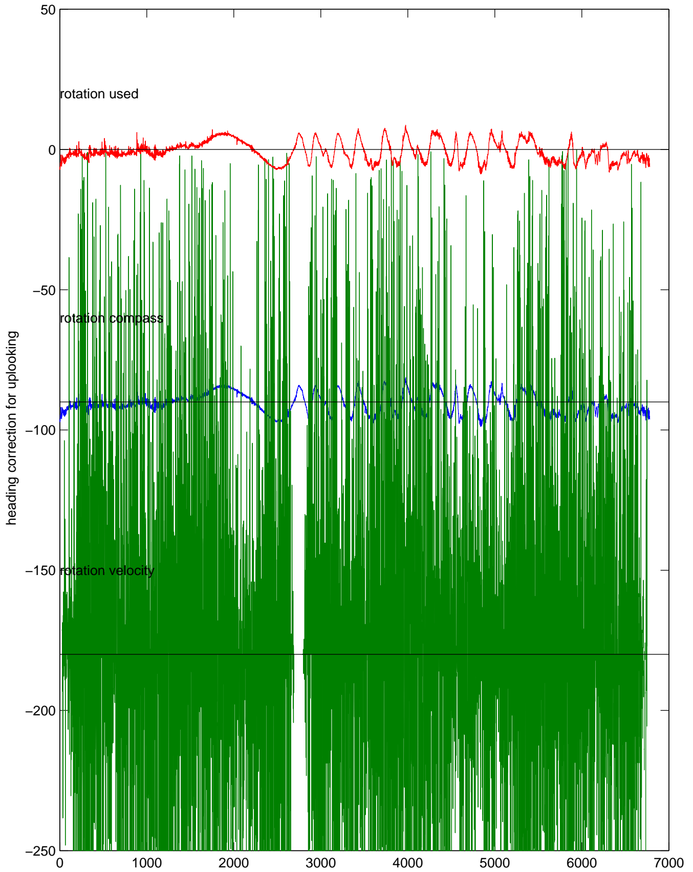
rh11751 (LADCP #188; V5) Figure 5
