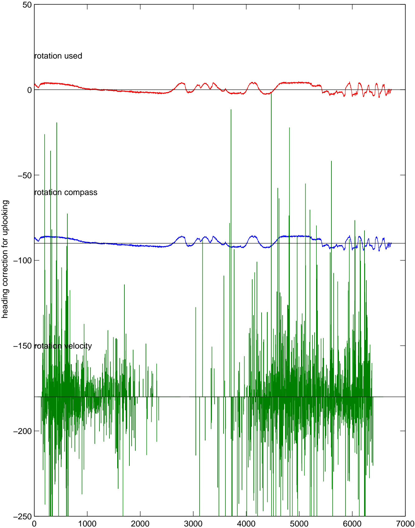
P16N station #173 (V7) Figure 5
