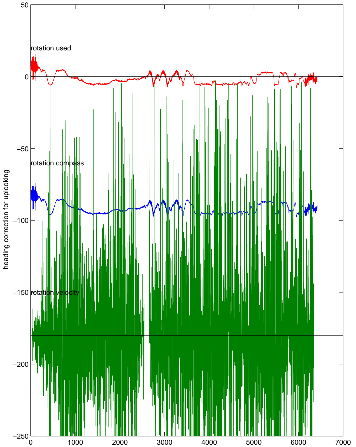
rh10571 (LADCP #065; V5) Figure 5
