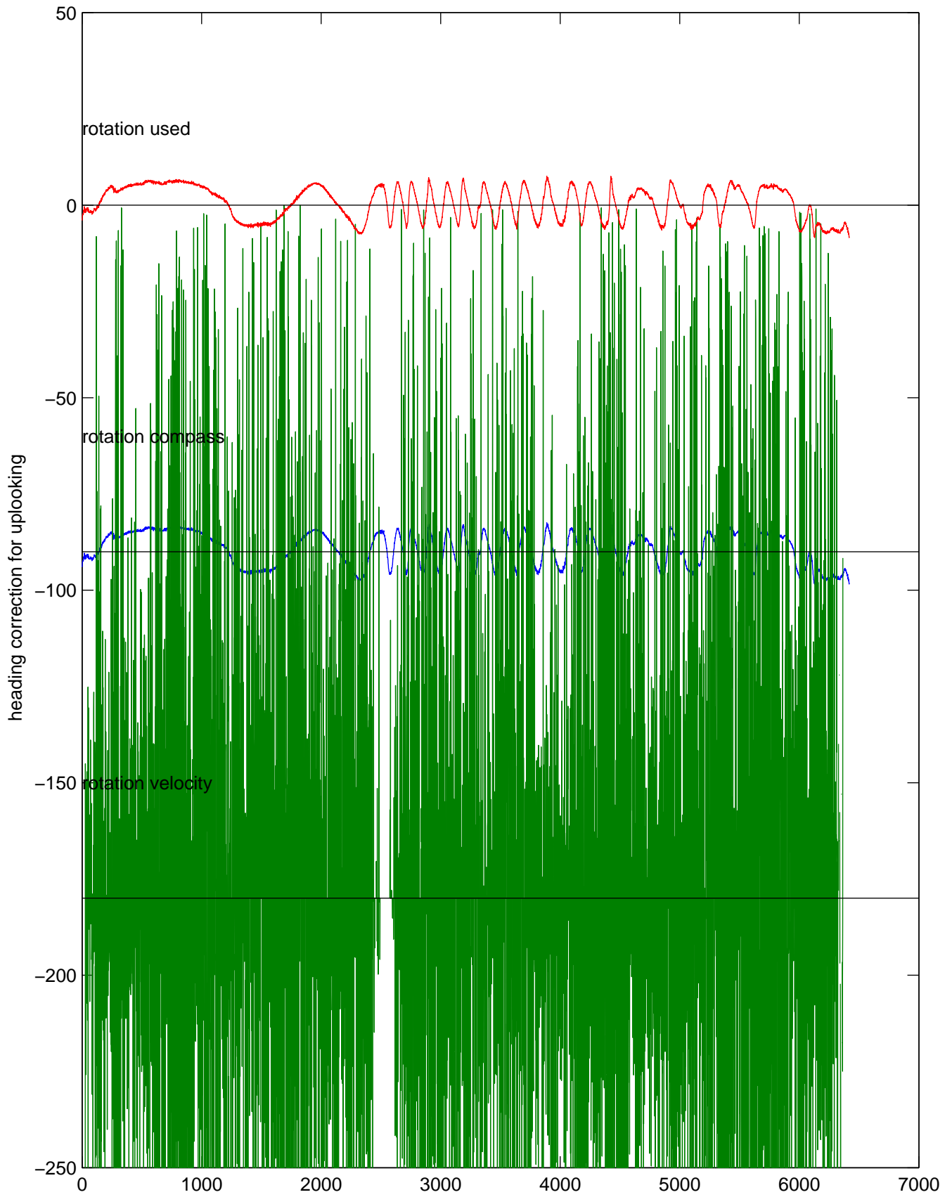
rh11601 (LADCP #172; V5) Figure 5
