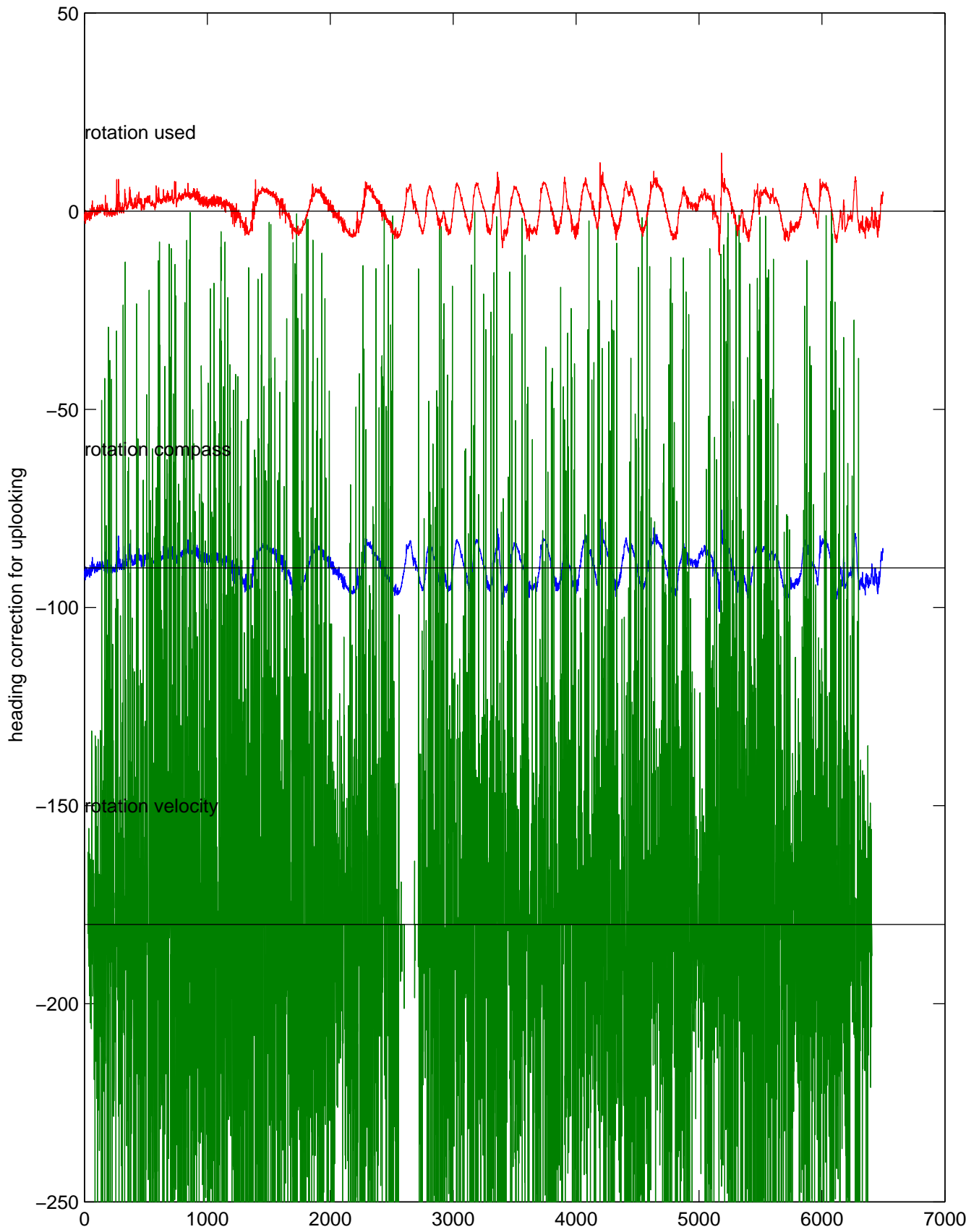
rh11671 (LADCP #180; V5) Figure 5
