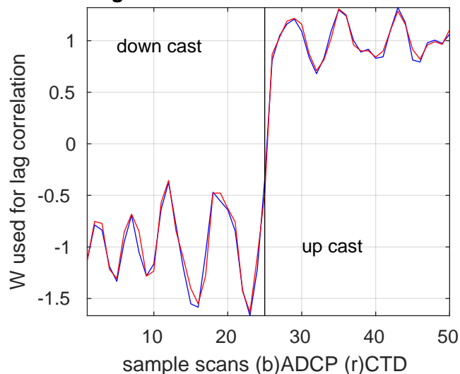
best lag W: 65 scans ~ -65 sec. c:0.99765
