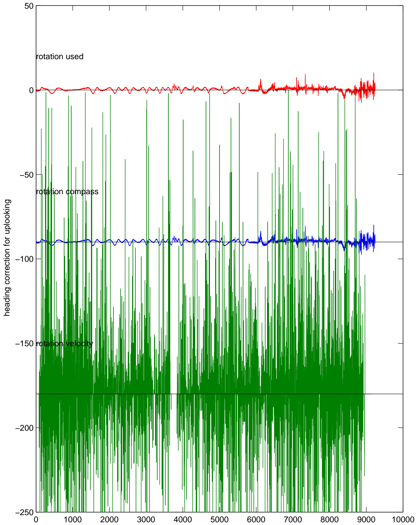
P16N station #20 (V7) Figure 5
