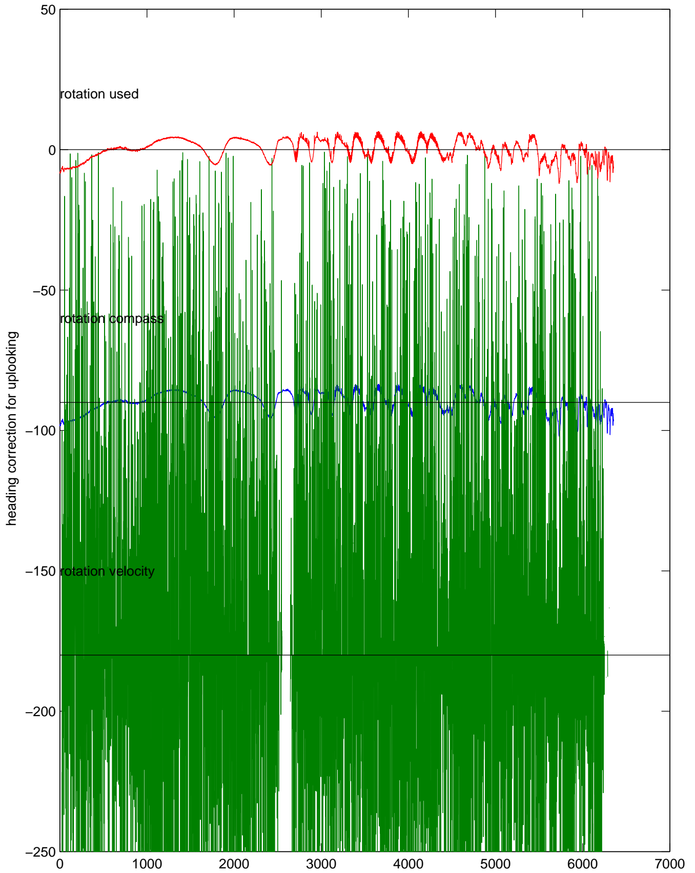
rh10911 (LADCP #099; V5) Figure 5
