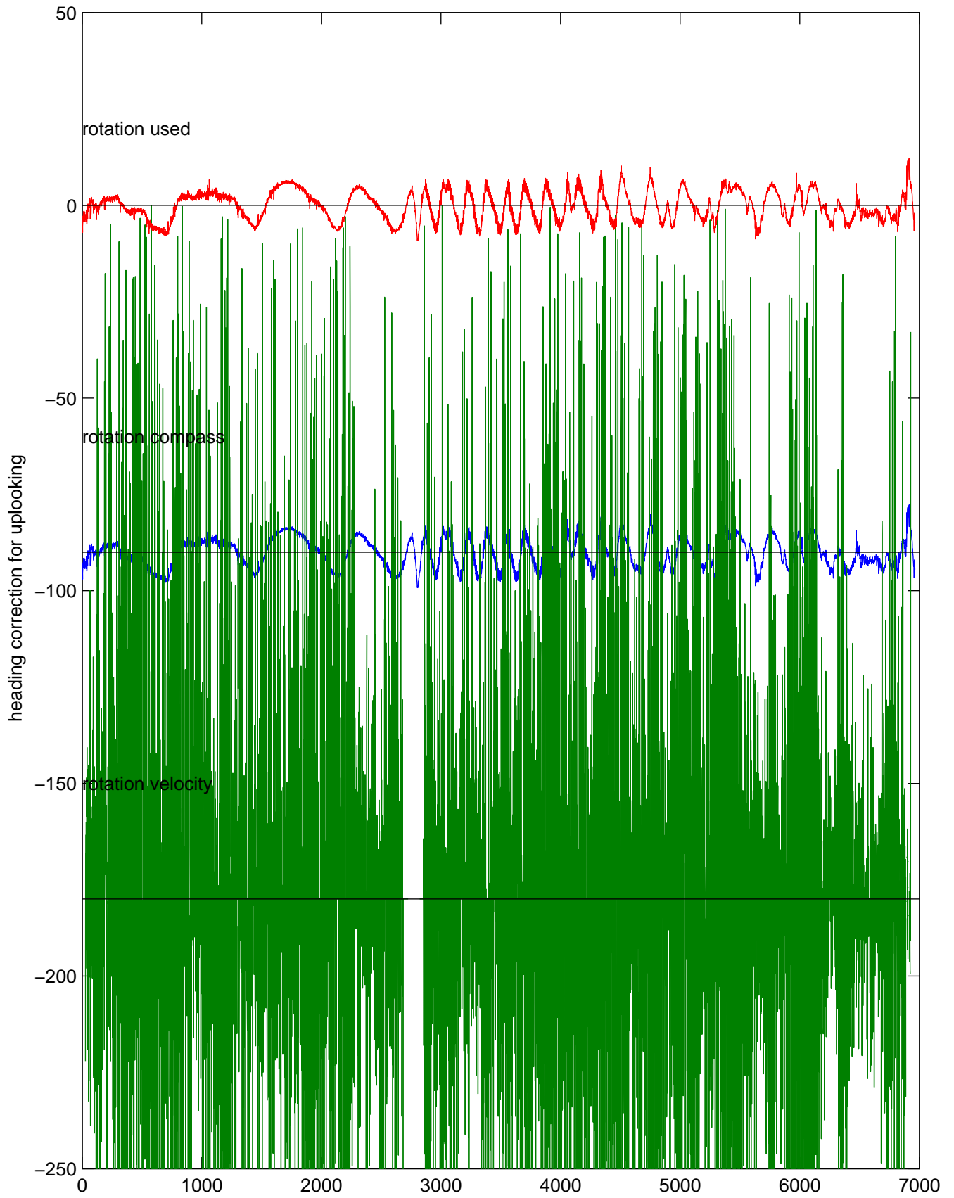
rh11661 (LADCP #179; V5) Figure 5
