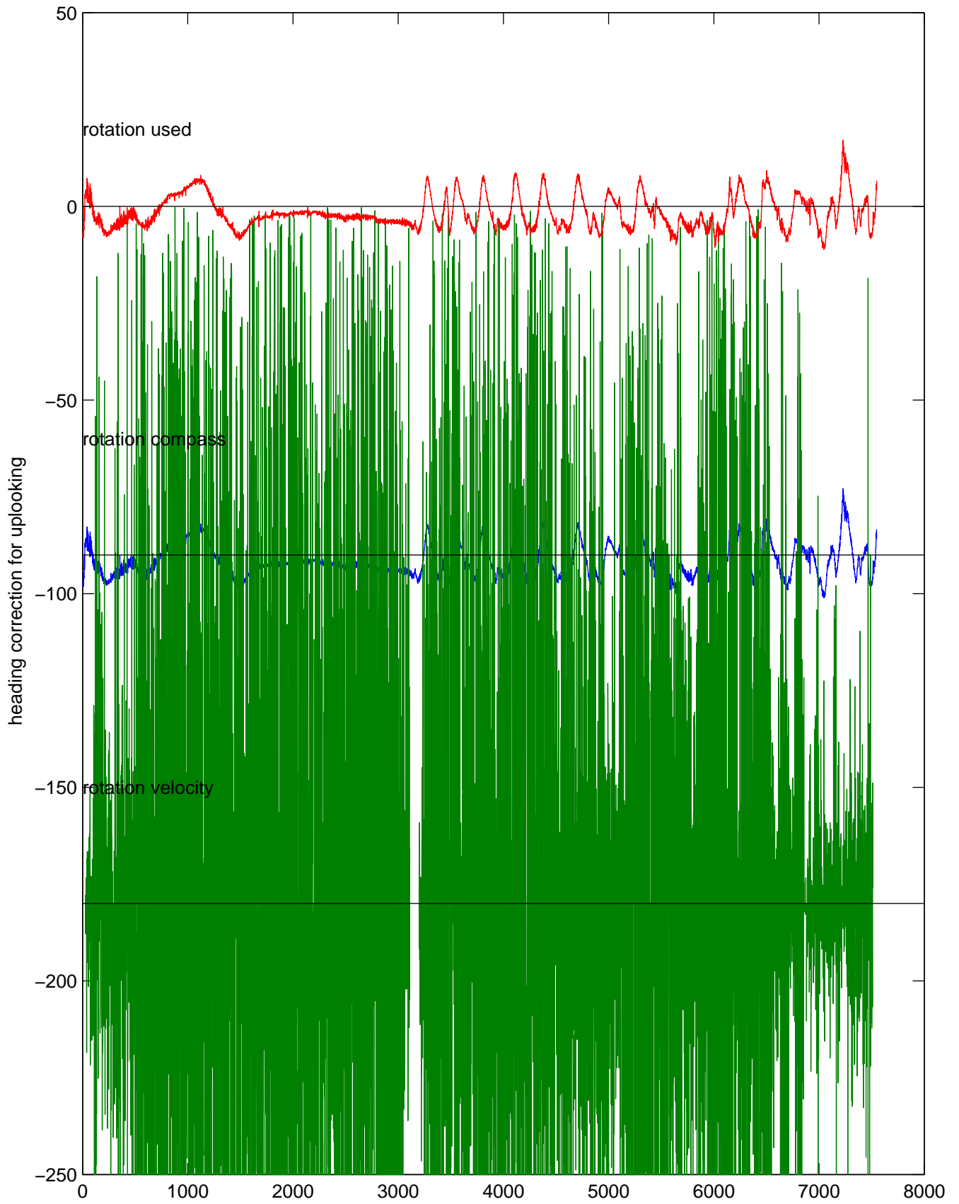
rh11991 (LADCP #212; V5) Figure 5
