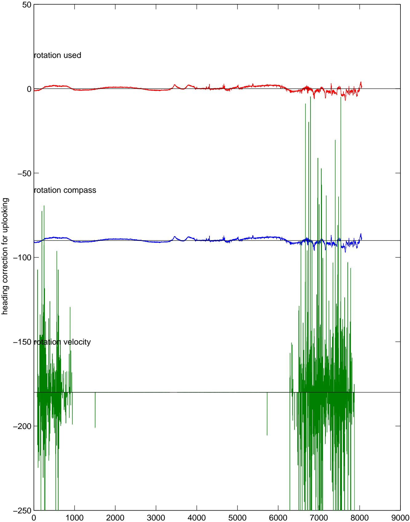
P16N station #121 (V7) Figure 5
