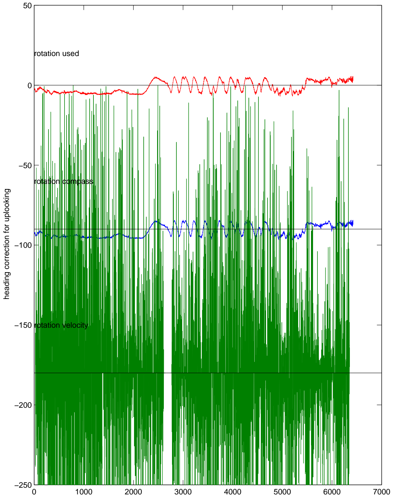
rh11041 (LADCP #112; V5) Figure 5
